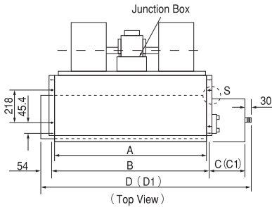
Figure 2 : HCCA Unit With Rear Return Plenum
