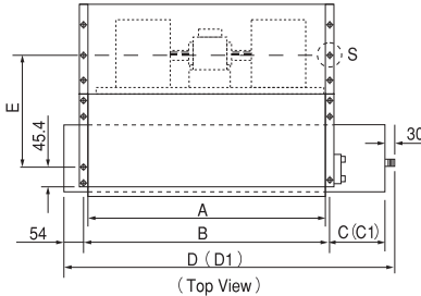
Figure 4 : S & T Drain Pan, For (Fig 1, 2, 3)
