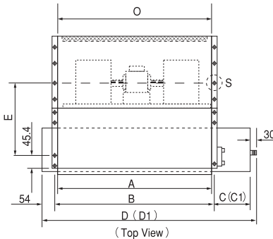
Figure 3 : HCCA Unit With Bottom Return Plenum
